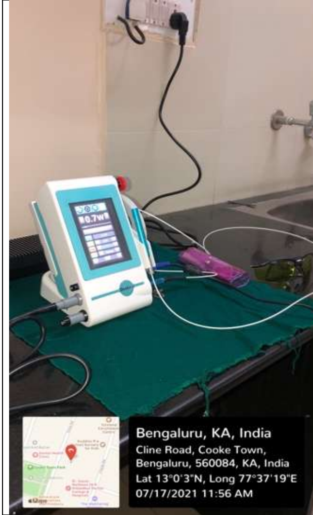
Soft Tissue Laser Unit
